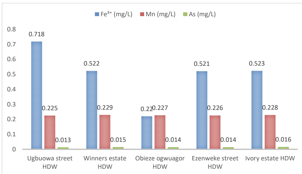
Figure 6: Metal Content in Water Samples from Different Locations in the Trans-Ekulu Area
