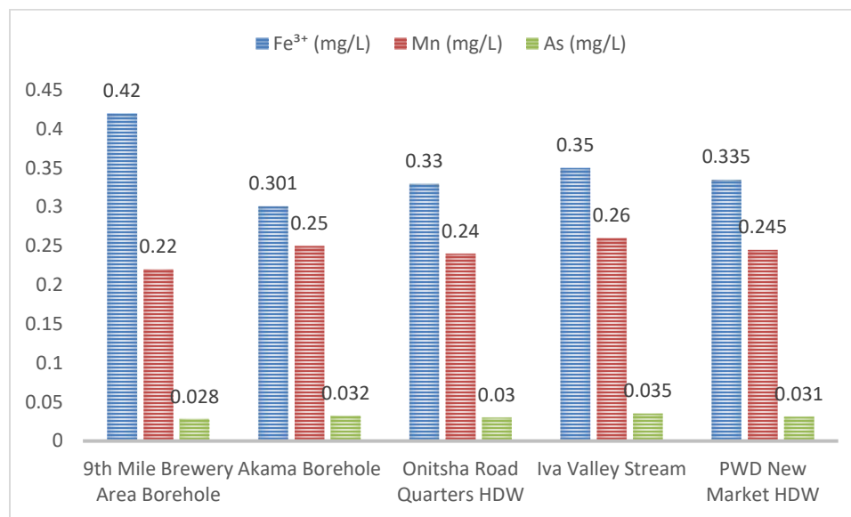
Figure 4: Metal Content in Water Samples from Different Locations in the Ajali River/9th Mile Area
