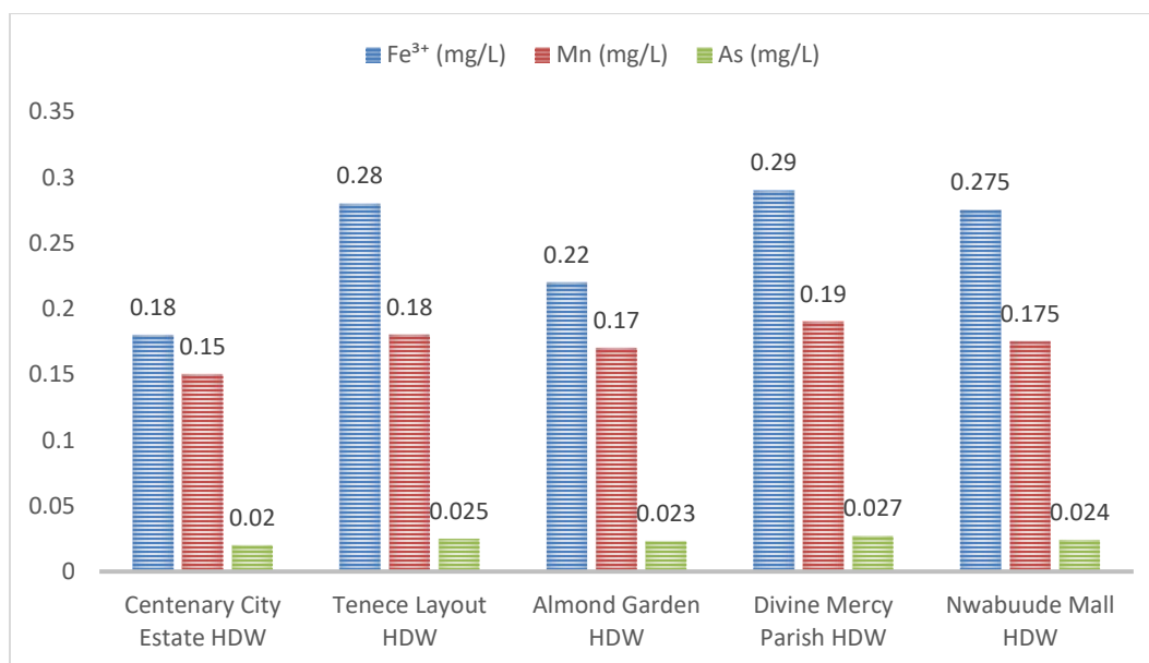
Figure 5: Metal Content in Water Samples from Different Locations in the Centenary Water Area
