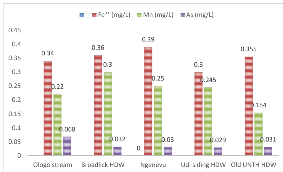
Figure 2: Metal Content in Water Samples from Different Locations in the Ologo Area
