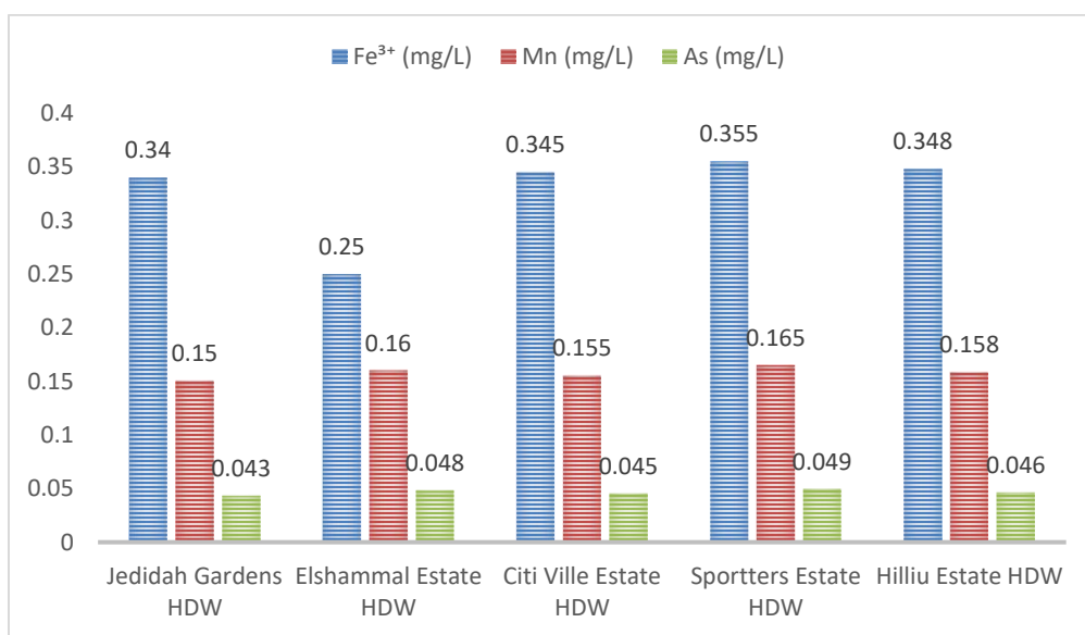
Figure 3: Metal Content in Water Samples from Different Locations in the Amechi Area
